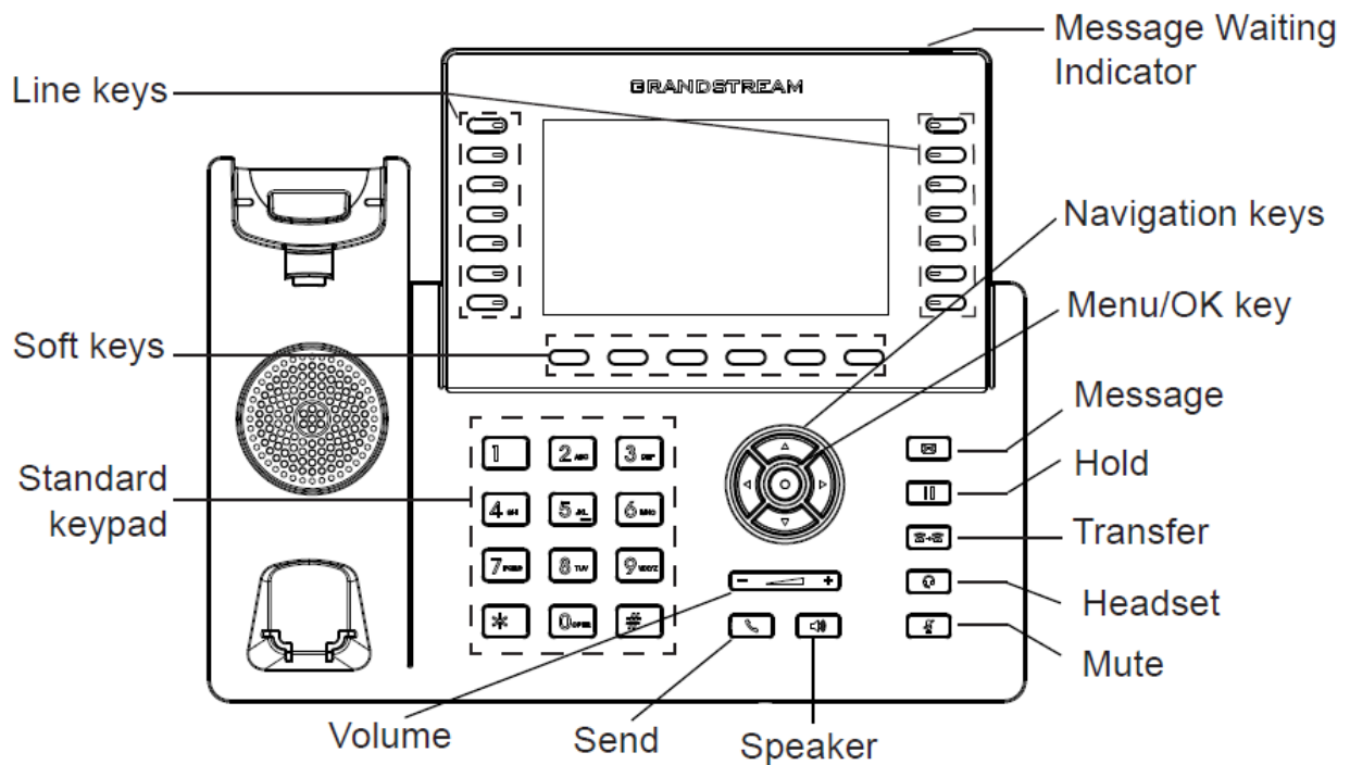
Figure 14: GRP2650 keypad
