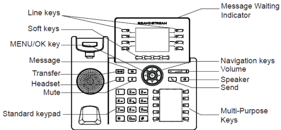
Figure 12: GRP2634 Keyboard
