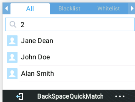
Figure 71: QuickMatch
