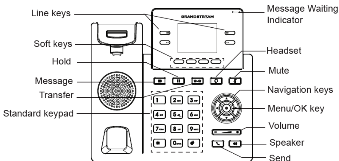
Figure 6: GRP2612/GRP2612P/GRP2612W/GRP2612G Keyboard
