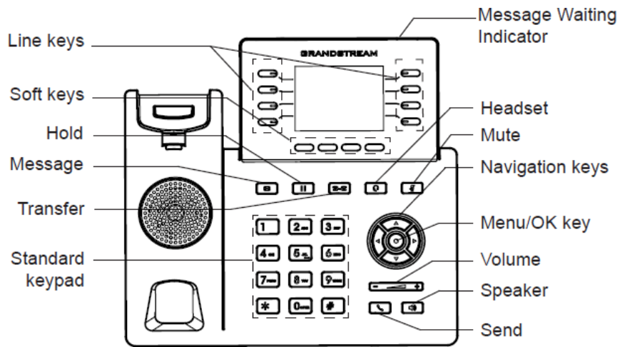
Figure 10: GRP2616 Keyboard
