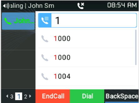
Figure 56: Predictive Dialing
