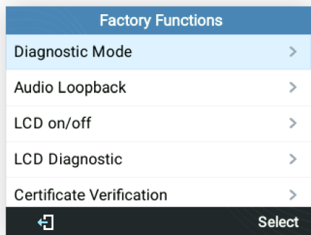
Figure 63: Factory Functions
