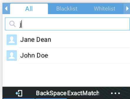
Figure 72: ExactMatch
