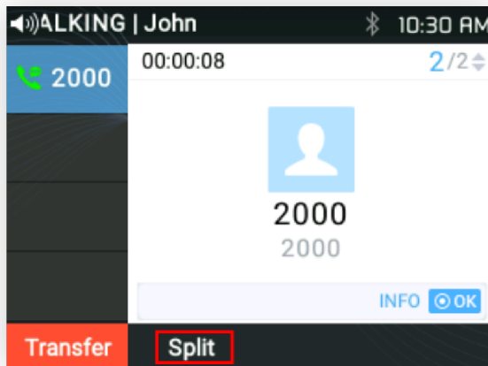
Figure 29: "Split" softkey
