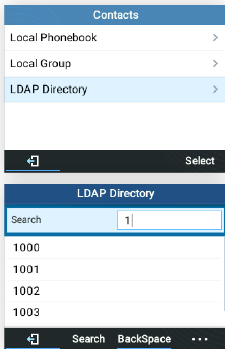
Figure 73: LDAP search
