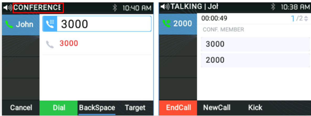
Figure 33: Established Conference
