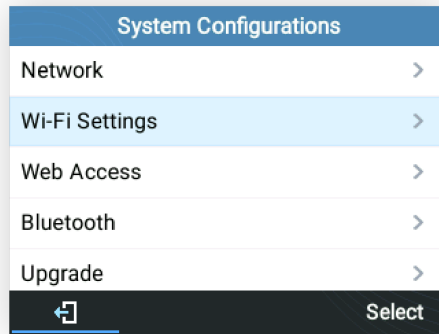
Figure 84: Wi-Fi feature
