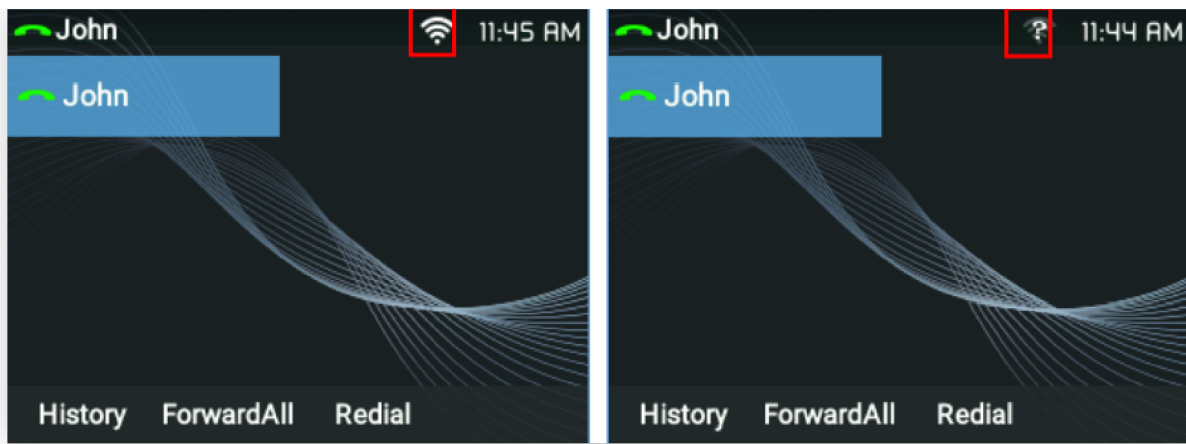
Figure 90: Wi-Fi Status
