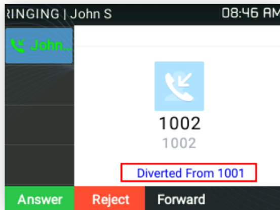
Figure 45: Diversion Information
