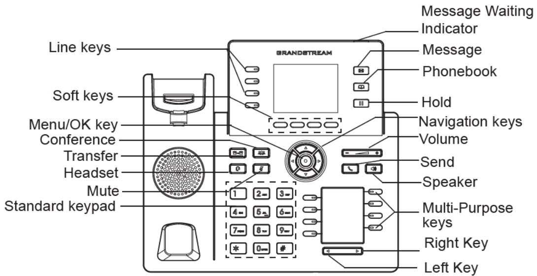
Figure 8: GRP2614 Keyboard
