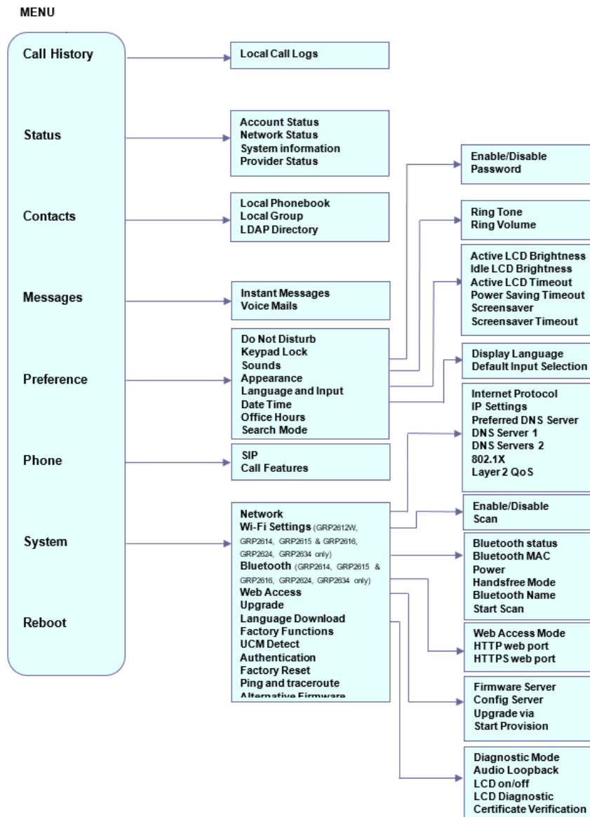
Figure 15: GRP2600 Menu
