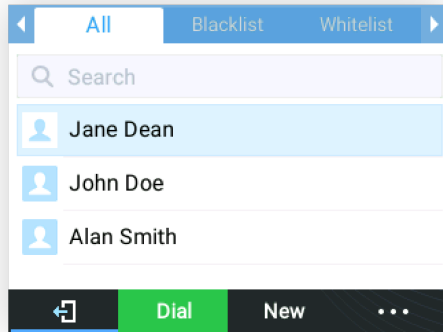
Figure 70: Before Search
