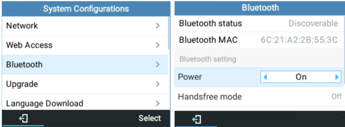
Figure 78: Bluetooth feature
