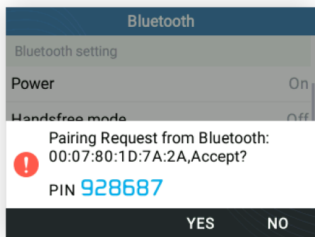
Figure 83: Pairing Request
