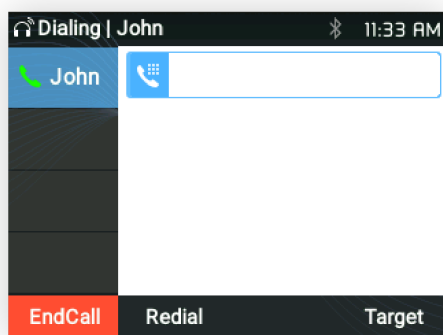
Figure 77: Headset enabled
