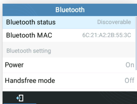
Figure 82: Bluetooth Status
