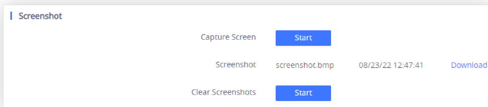
Figure 62: Screenshots
