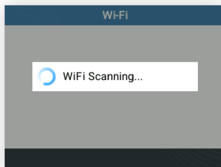
Figure 86: Wi-Fi Scanning
