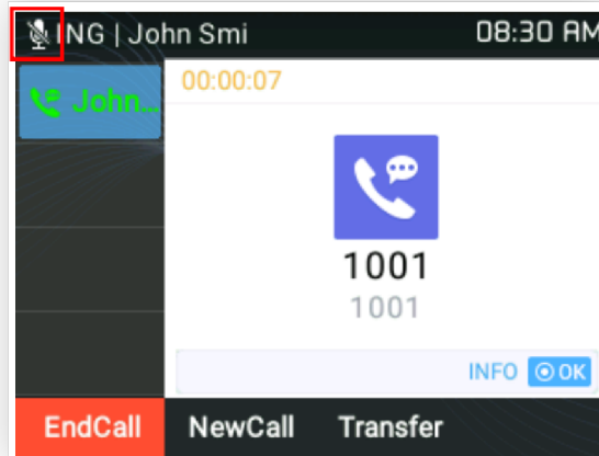
Figure 25: Call Muted
