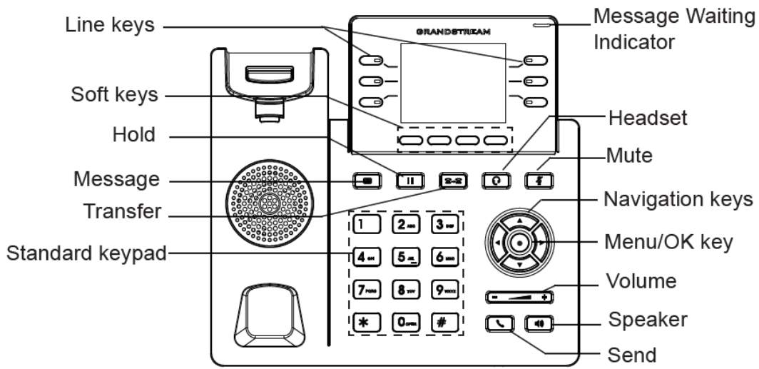
Figure 7: GRP2613 Keyboard
