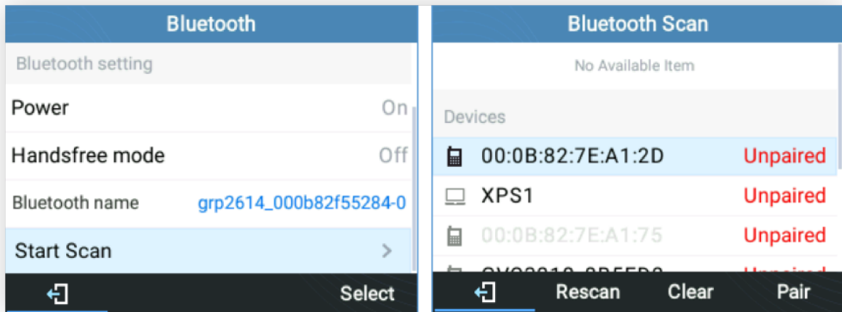
Figure 79: Bluetooth Scan
