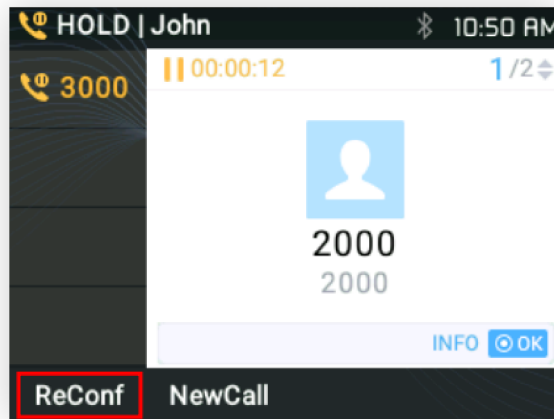
Figure 35: Split conference
