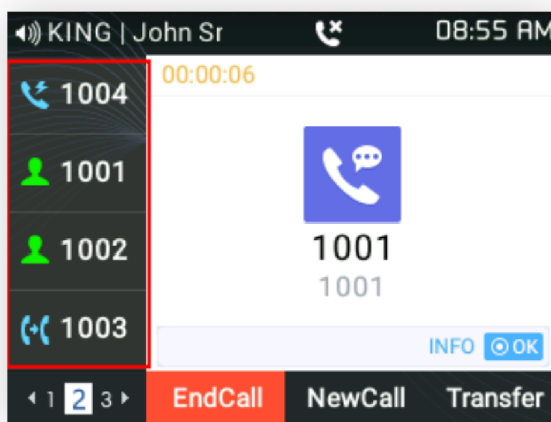
Figure 59: VPK Paging
