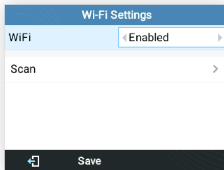
Figure 85: Enable Wi-Fi
