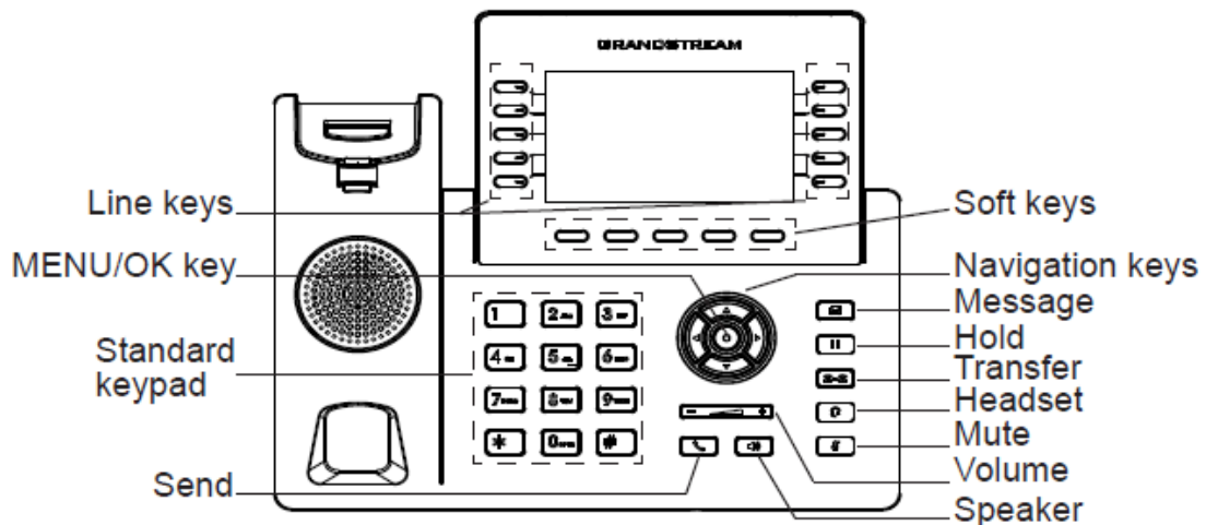
Figure 9: GRP2615 Keyboard
